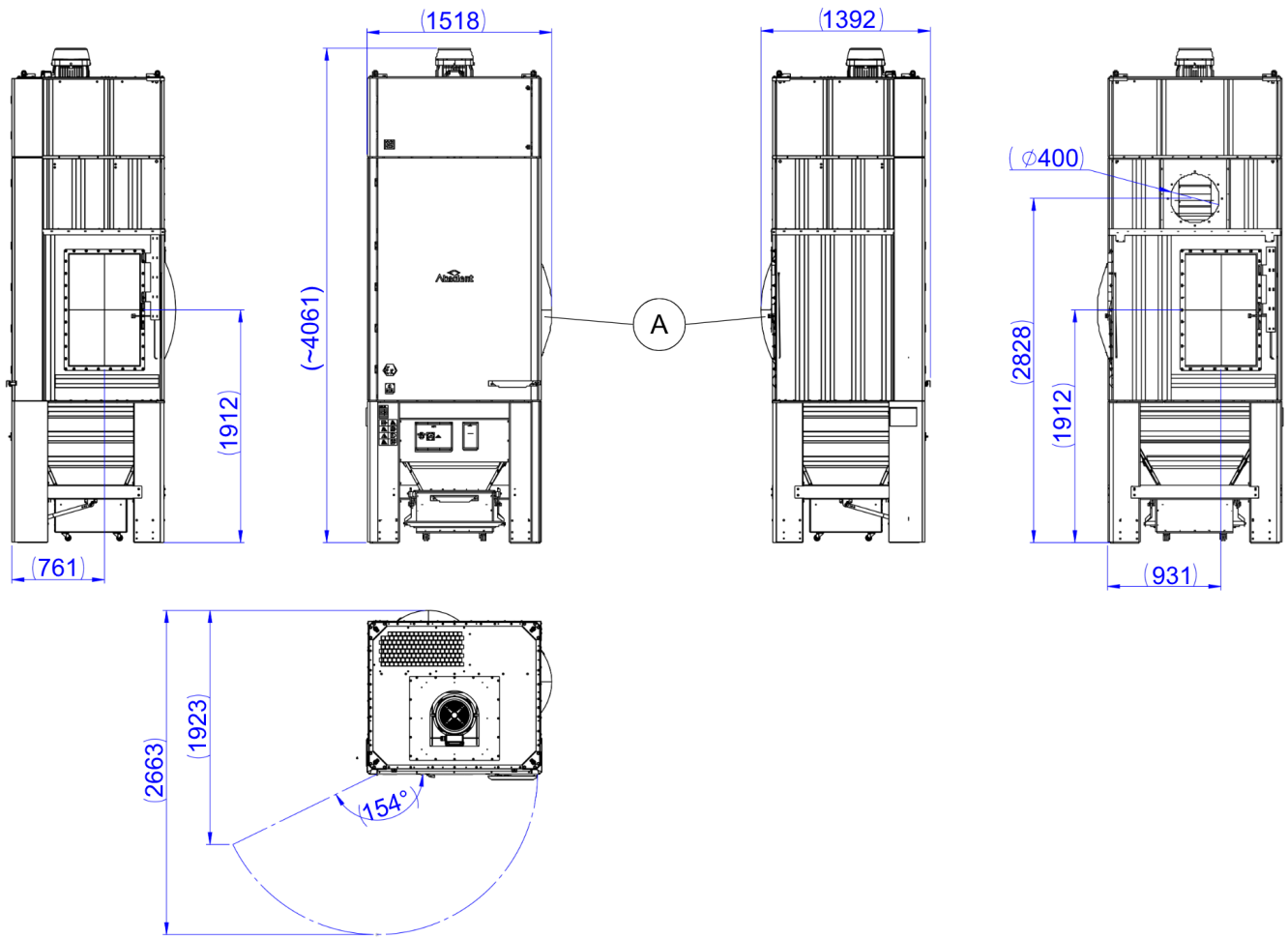
AD101EX with integrated fan and two explosion panels (A).
