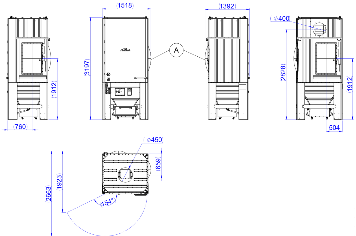
AD101EX with external fan and two explosion panels (A).
