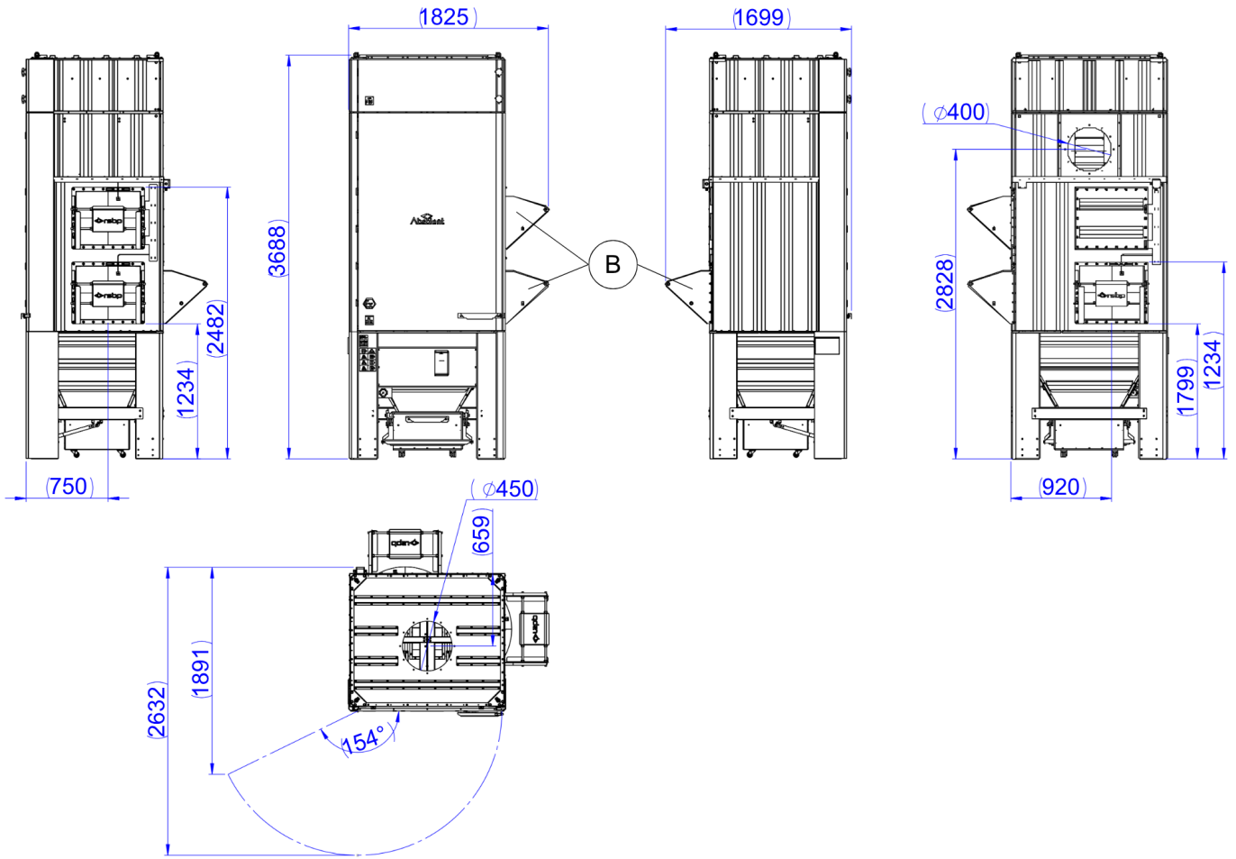
AD101EX with external fan, three explosion diverters (B) and HEPA module.
