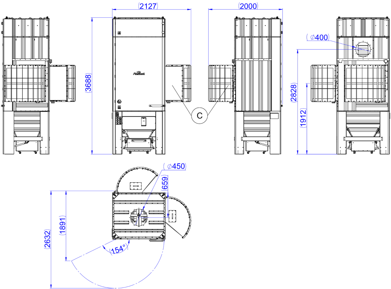
AD101EX with external fan, HEPA module and two flameless vents (C).
