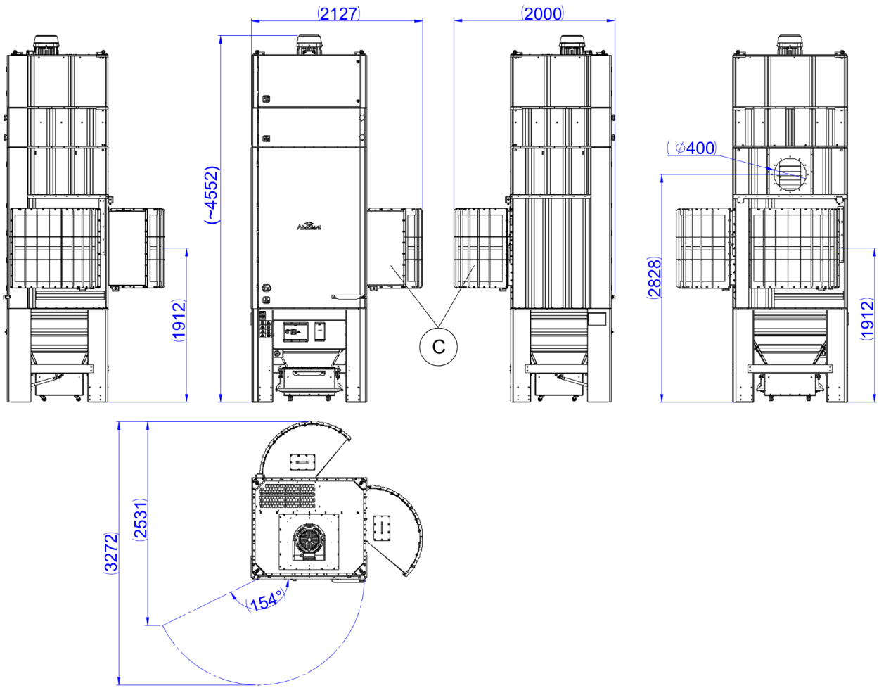
AD101EX with integrated fan, HEPA module and two flameless vents (C).
