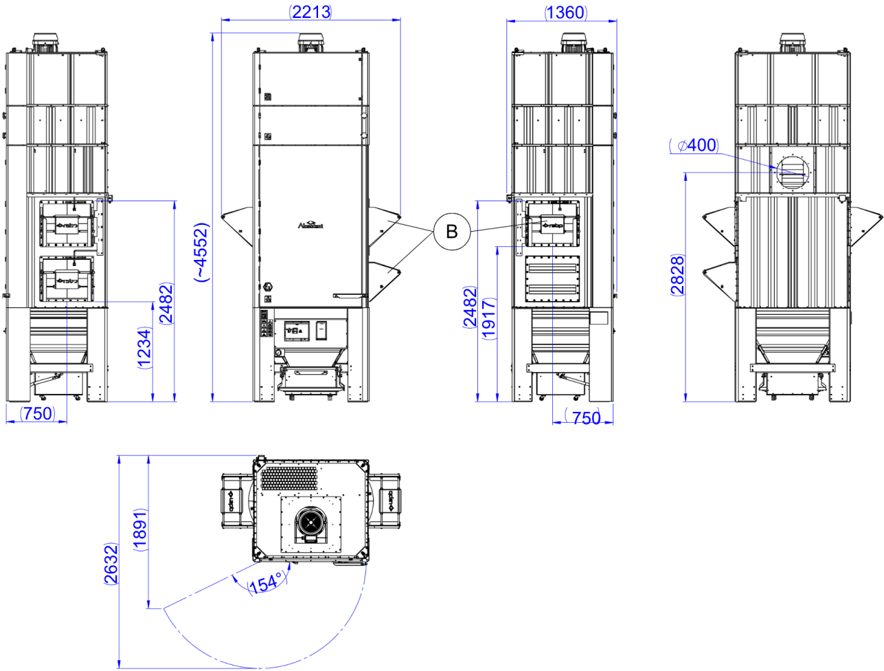
AD101EX with integrated fan, three explosion diverters (B) and HEPA module.
